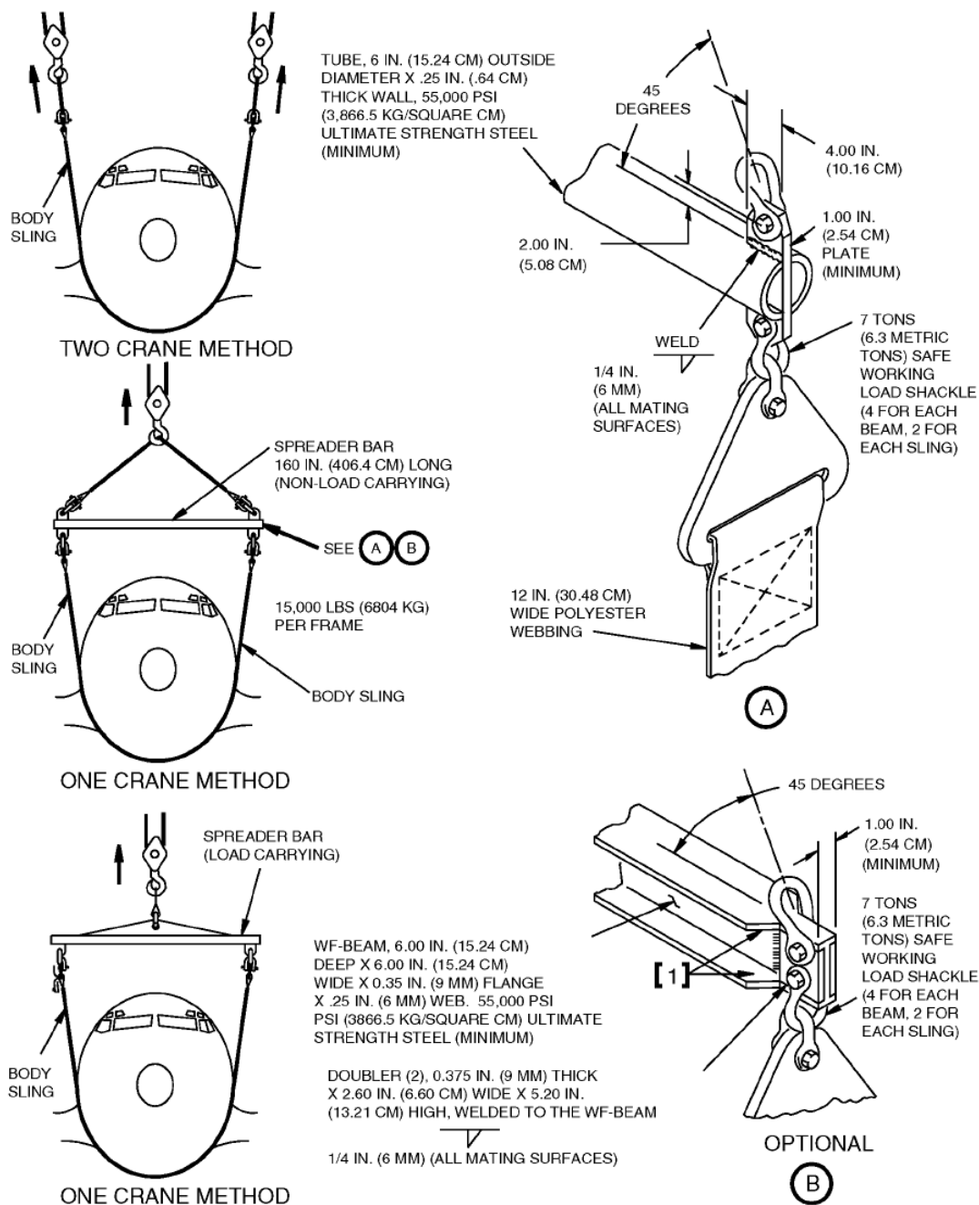
Figure 3-60 LIFTING THE NOSE WITH A SLING
