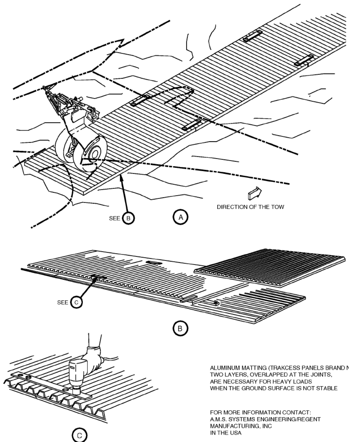
Figure 2-8 EXAMPLES OF PREPARED SURFACES (Continued)
