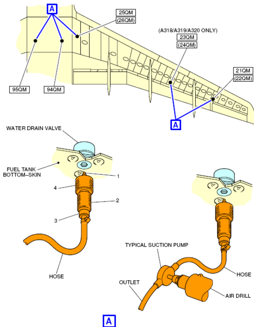
Drain Remaining Fuel Purging Tool Installation FIGURE-05-40-02-991-004-A01
